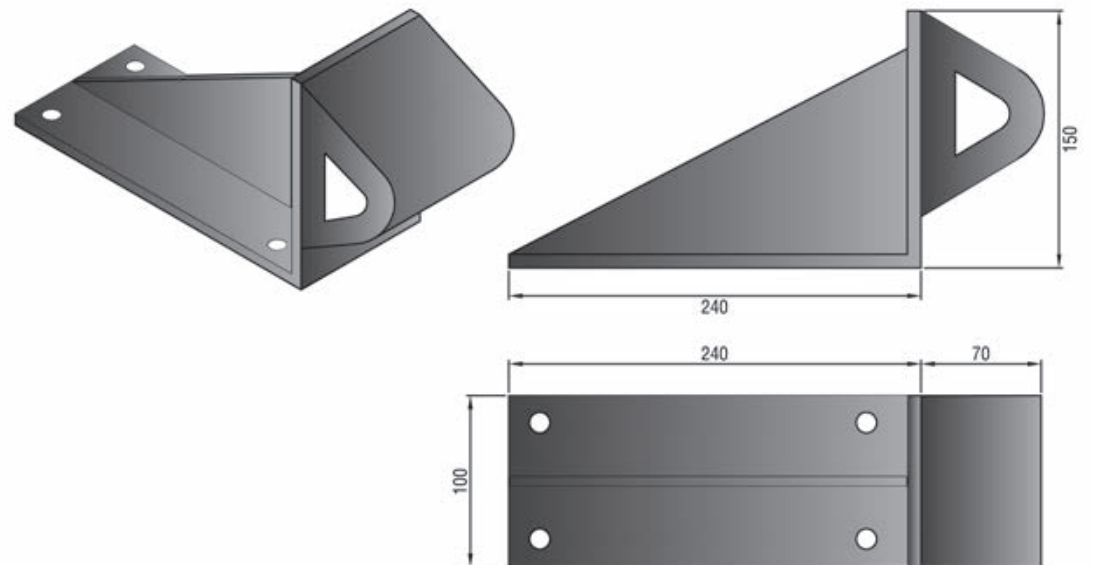
49 - Heavy Duty industrial door stop. Floor Mounted.
