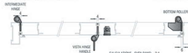
2 LEAVES FOLDING TO ONE SIDE
