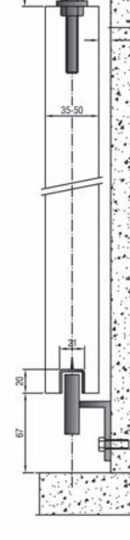
ALTERNATE GUIDING 19S STEEL CHANNEL RECESSED UNDER DOOR WITH 5012H STEEL GUIDE.
