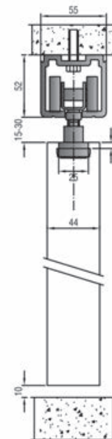
SOFFIT FIX 400TA TRACK WITH 400TP/T HANGER ON TIMBER DOOR
