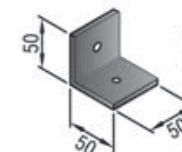
A200 steel bracket for 200A track
