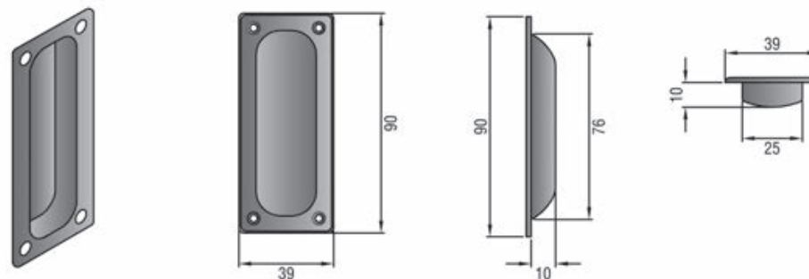
502 FLUSH HANDLE - Aluminium (natural, gold anodised)
