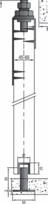
ALTERNATE GUIDING 25S STEEL CHANNEL RECESSED UNDER DOOR WITH 5016 STEEL GUIDE.
