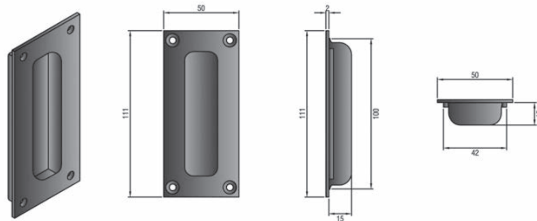
503SL FLUSH HANDLE - Aluminium (natural, gold, bronze anodised)
