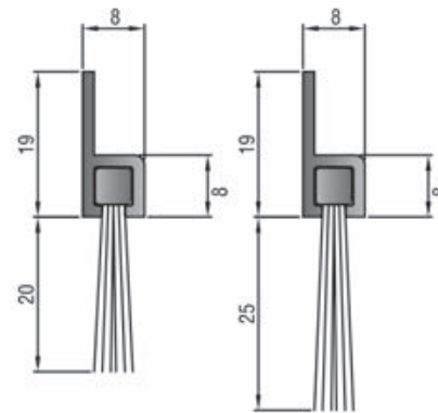
122 BRUSH WELT - ALUMINIUM CARRIER WITH POLYPROPYLENE BRUSH
