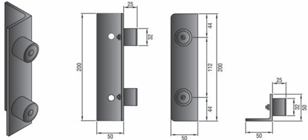
49 - Heavy Duty industrial door stop. Floor Mounted.
