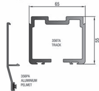
200TA 400TA, 356TA & 600TA TRACK LENGTHS 1.5m; 2m; 2.5m; 3m; 3.5m; 4m; 5m; 6m
