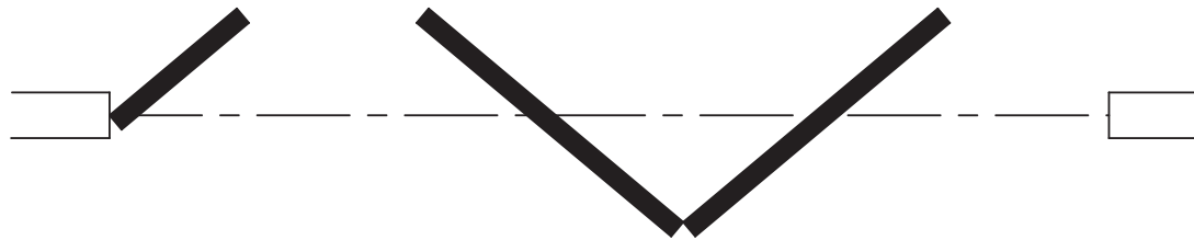
SLIDING AND FOLDING TO ONE SIDE - PARTITIONFOLD (CENTRE HUNG IN PAIRED PANELS WITH HINGED LEAF)
