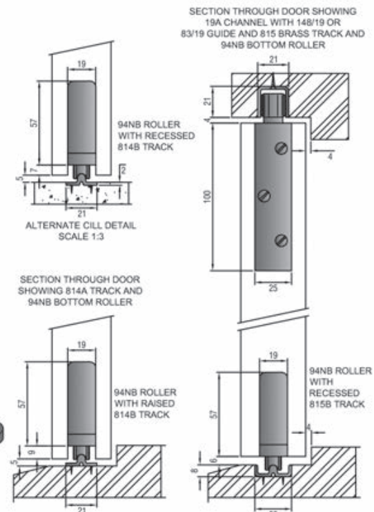
ALTERNATE CILL DETAILS SCALE 1:3
