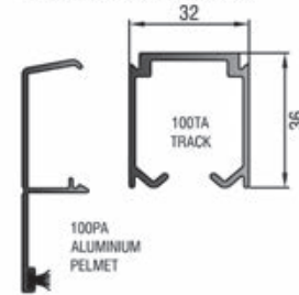
100TA TRACK LENGTHS 1.5m; 2.1m; 2.4m; 3m; 3.6m; 6m; 7.2m
