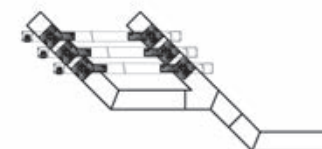
45DEG CRANKED STAGGERED STACK - LH/RH
