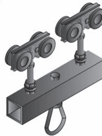
W468 - 8 WHEEL HANGER
