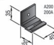
A100 steel bracket for 100 steel track
