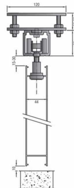
SECTION THROUGH DOORS SECTION SCALE: 1:4
