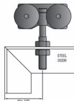
A1000LJ SIDE FIX LOCK JOINT BRACKET
