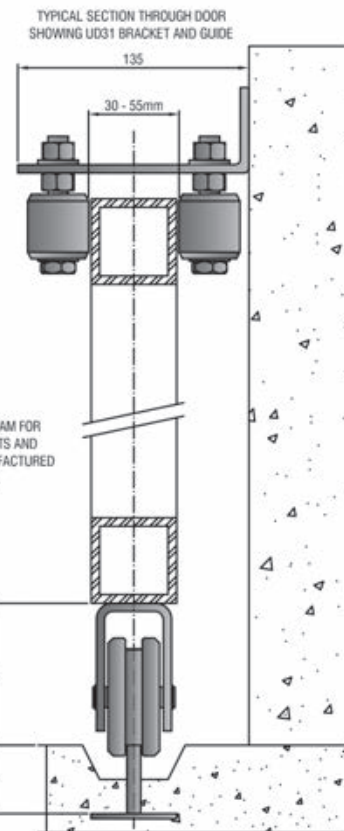
GWR50/60F BOTTOM ROLLER ON 50x50 SQUARE WITH RECESSED 408 BOTTOM STEEL TRACK
