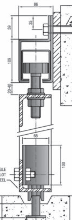
SECTION THROUGH DOOR SHOWING ALTERNATE CILL DETAILS OF 0832 BOTTOM ROLLER WITH RAISED AND RECESSED 5012 STEEL TRACK SCALE 1:5
