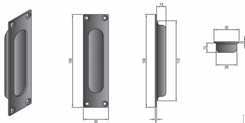
503SL FLUSH HANDLE - Aluminium (natural, gold, bronze anodised)
