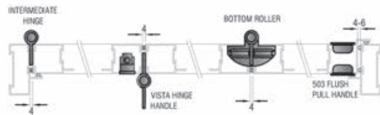
3 LEAVES FOLDING TO ONE SIDE
