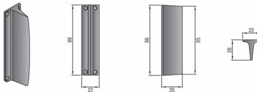
96TP HANDLE - Plastic
