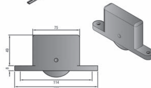
94NB MORTICE FIX ROLLER (2 PER DOOR)
