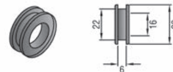
H208 FINGER PULL - Chromed plastic (22mm DIA HOLE IN GLASS)
