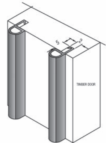
TEG TIMBER SEAL
