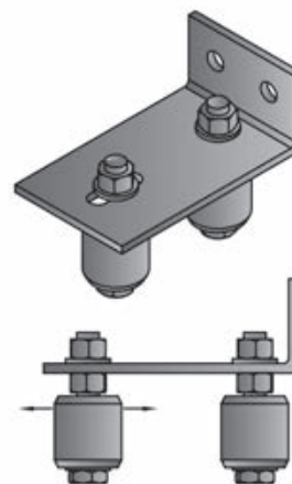
UD31 BRACKET AND GUIDE 30 - 55mm ADJUSTMENT
