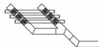
45DEG CRANKED STAGGERED STACK - LH/RH
